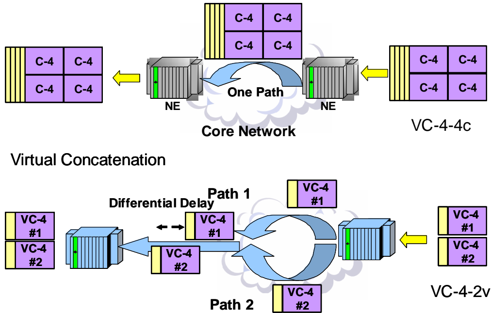
Fig. 5 Virtual & Contiguous Concatenation
